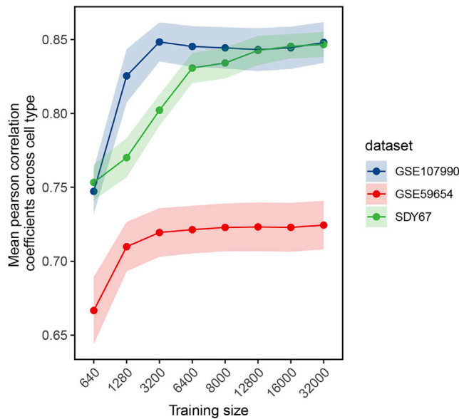
Figure 6. Assessment of the effect of training data size on mean Pearson correlation coefficients across cell types
