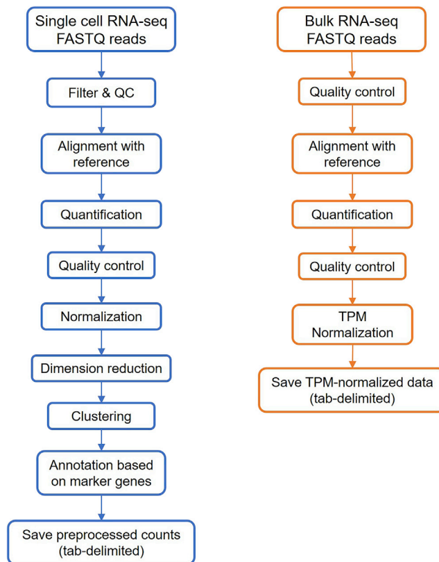
Figure 2. Schematic of preprocessing of single cell RNA-seq and bulk RNA-seq of purified cells
