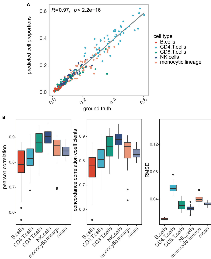
Figure 5. Performance evaluation of DAISM-DNN on RNA-seq dataset SDY67
